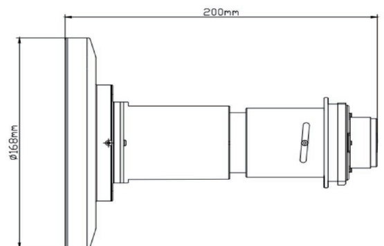
Outline Dimensions Drawing
